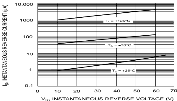
Fig. 7 Typical Reverse Characteristics, B350/A/B thru B360/A/B
