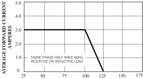
T , TERMINAL TEMPERATURE ( C )° Fig. 1 Forward Current Derating Curve
