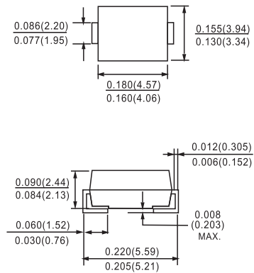
DO-214AA(SMB)
