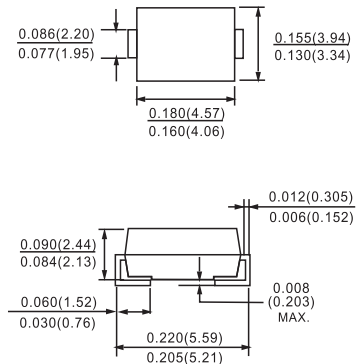
DO-214AA(SMB)
