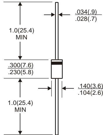
DO-15
